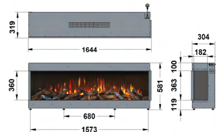
1650 -RIGHT CORNER
