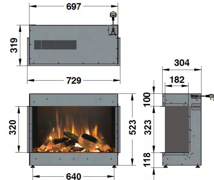
950 LT - BAY
