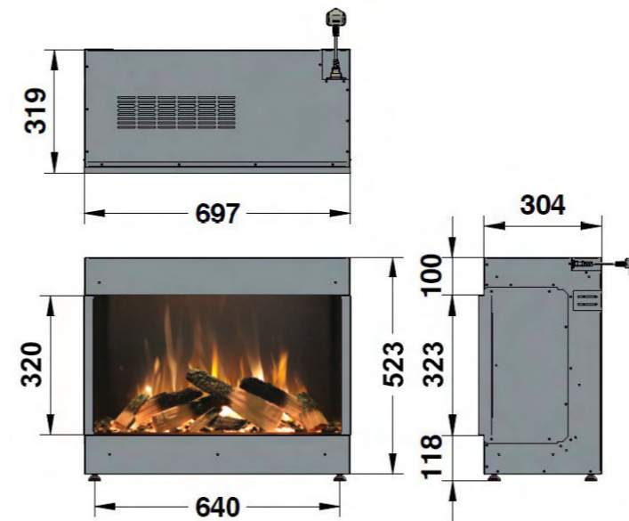
950 LT - FRONT
