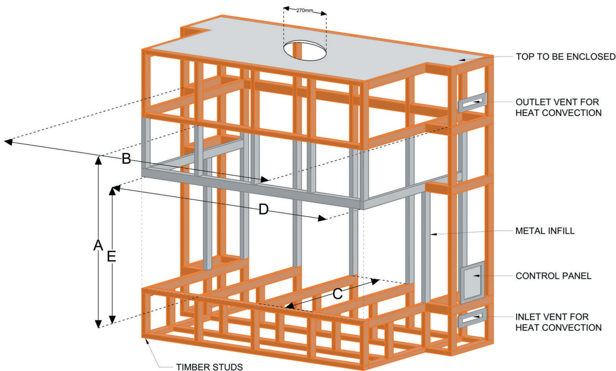
Figure 1.8 (Timber framing)
