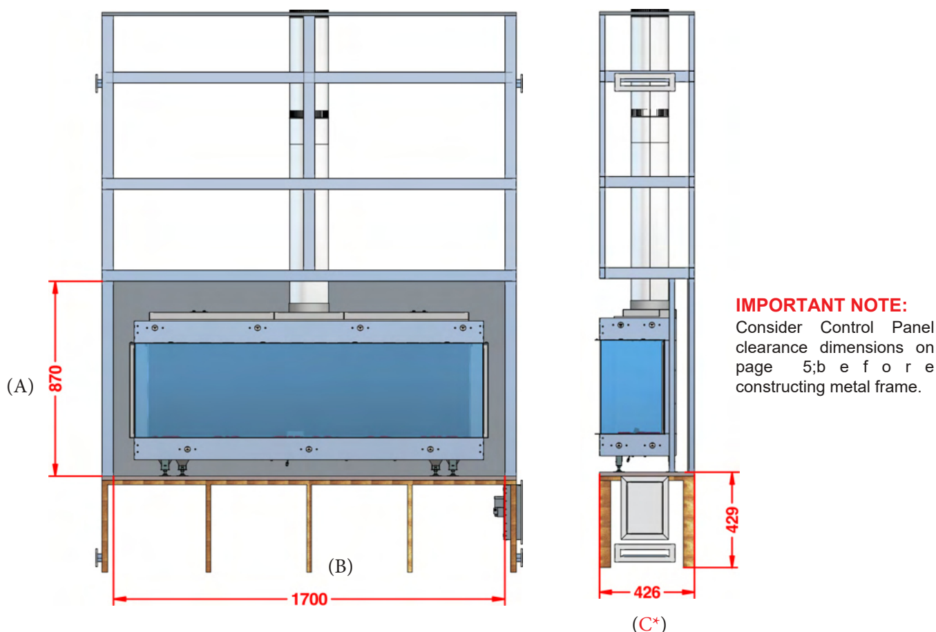
Figure 1.8 (Metal framing)
