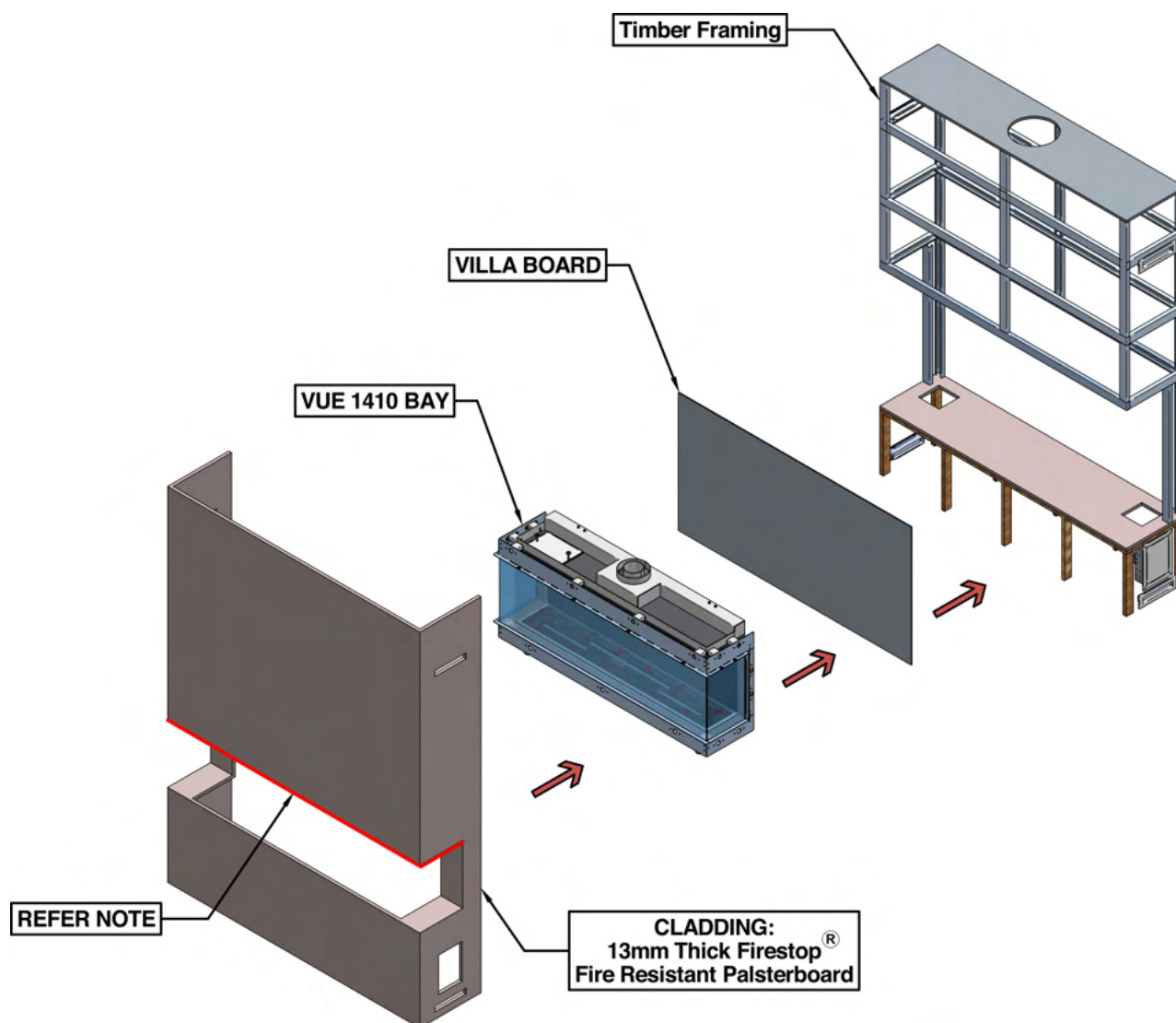
Figure 1.7 (Cladding Material)
