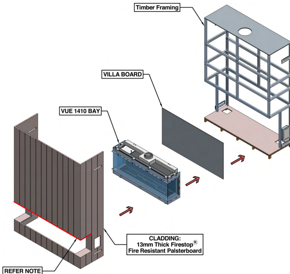
Figure 1.7 (Cladding Material)
