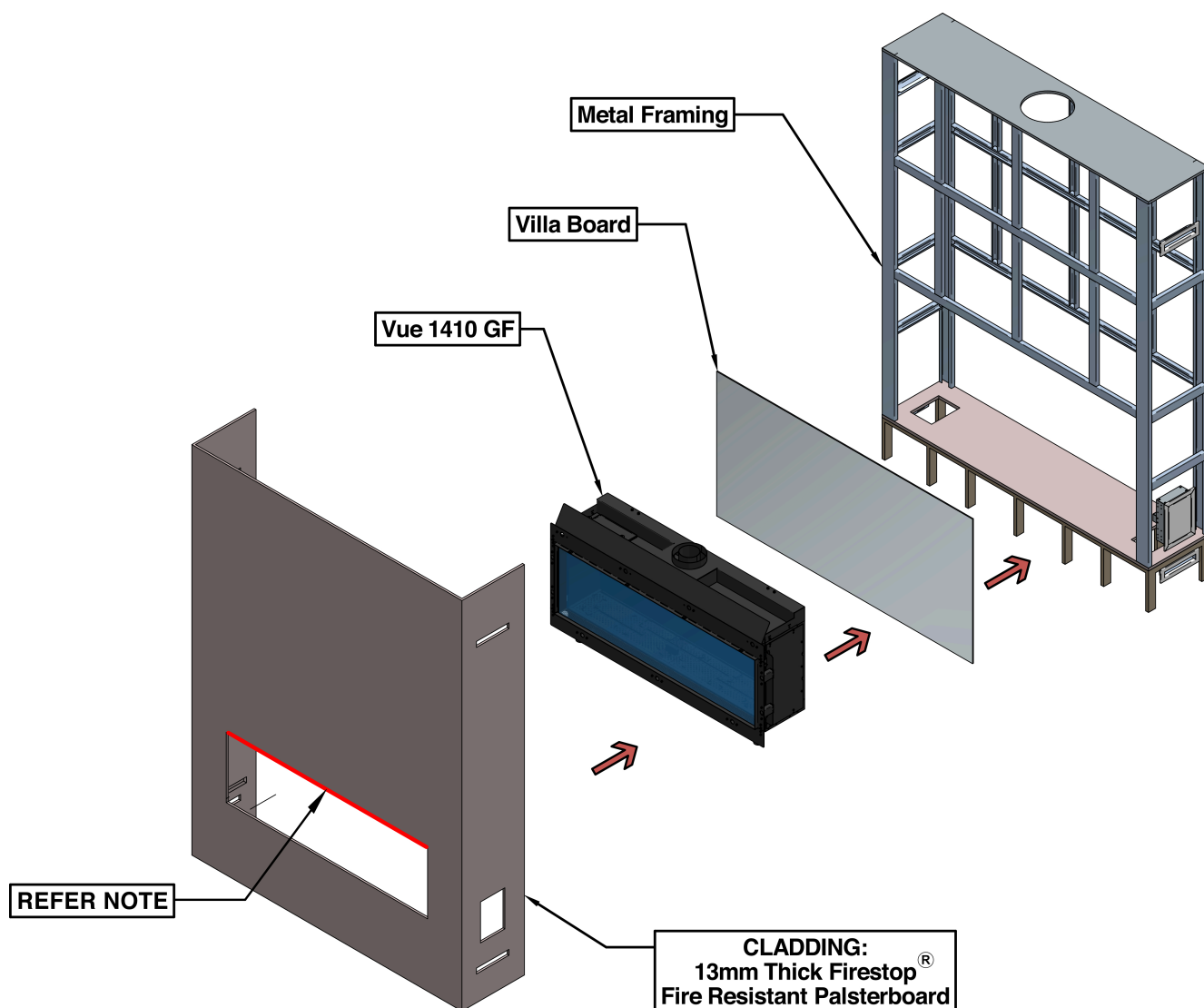
Figure 1.7 (Cladding Material)
