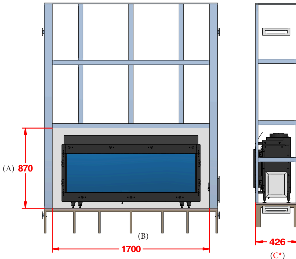
Figure 1.8 (Metal framing)
